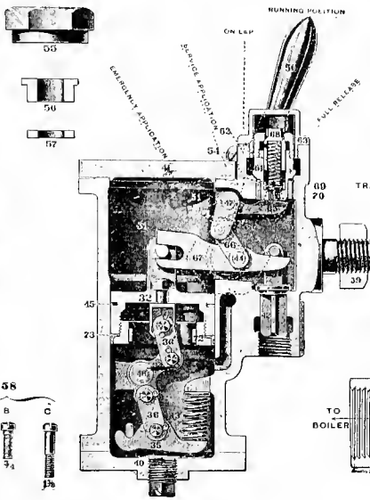
Fig. 1754. Section.
